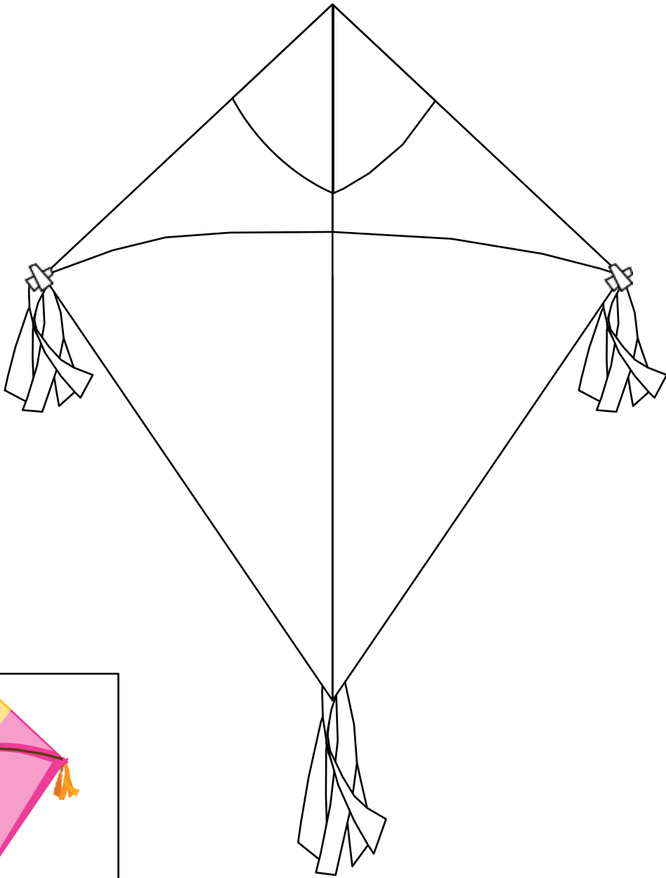
Kite
