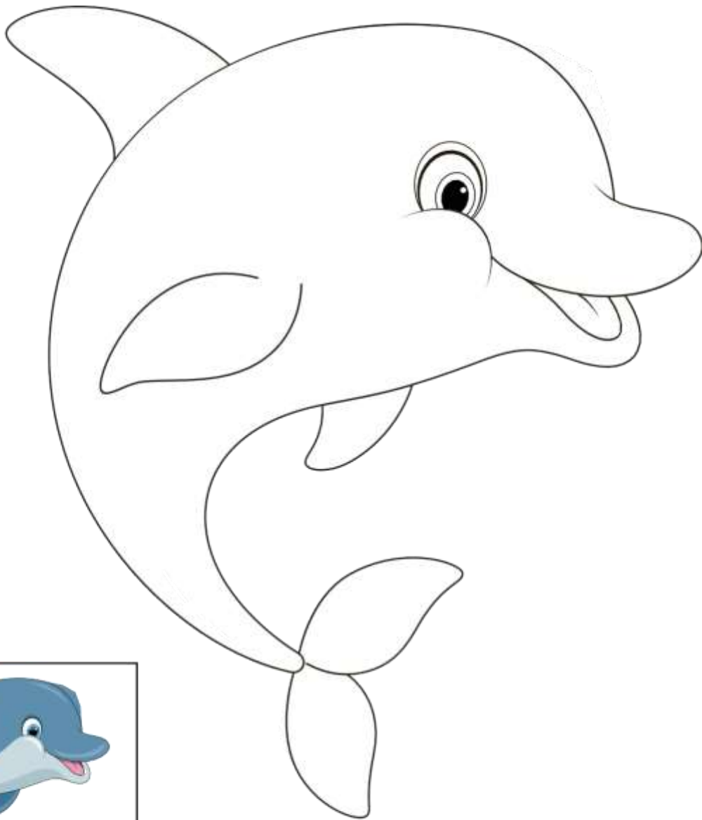
Dolphin
